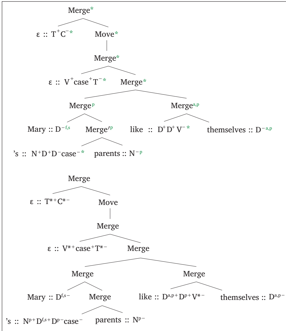
Figure 7: Converting a state assignment for a derivational version of Principle A into refined categories.
