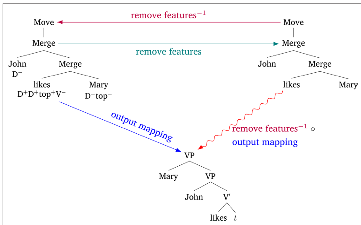
Figure 4: General procedure for constructing a feature-free MG.
