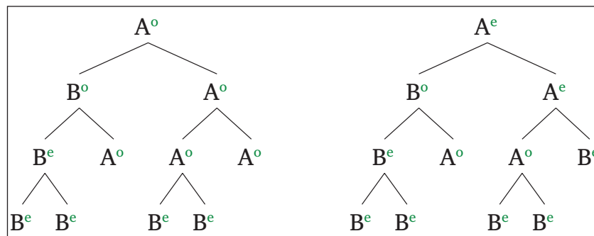
Figure 5: State assignments of the odd/even automaton for licit and illicit trees.
