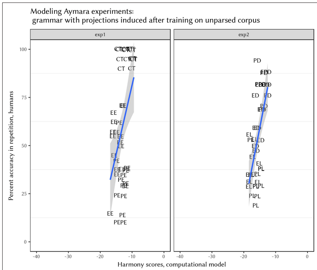
Figure 5: The Induced Unparsed Model: a grammar with induced projections built from the unsegmented corpus, tested on Aymara experimental data. Data points are labeled according to stimulus type; Exp. 1: “CT” is control, “PE” is plain-ejective, “EE” is ejective-ejective. Exp. 2: ED: ejective-ejective-dental, EL: ejective-ejective-labial, PD: plain-ejective-dental, PL: plain-ejective-labial).
