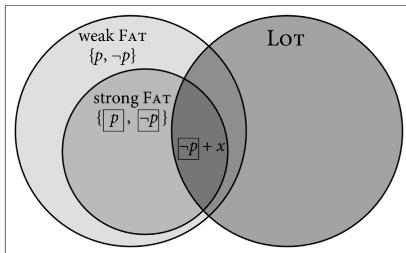
Figure 1: The relation between weak FAT, strong FAT, and (a specific) LOT.
