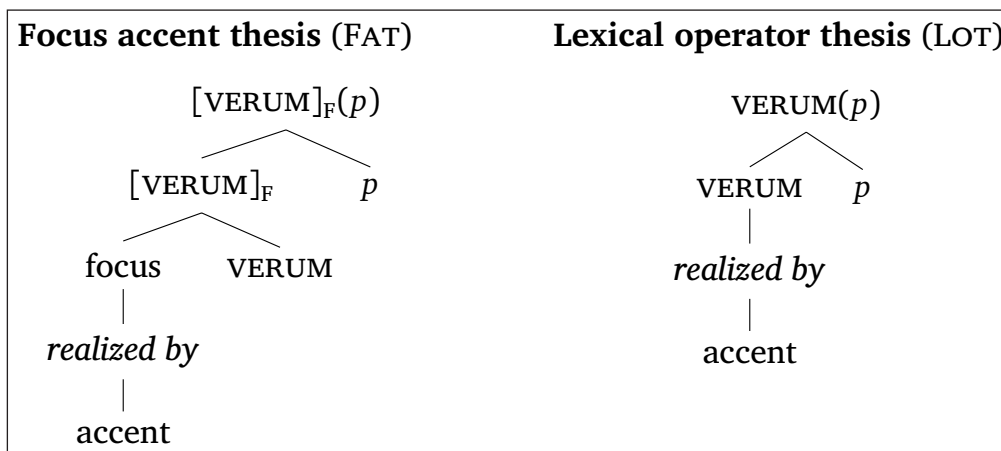
Figure 2: Comparing the FAT and LOT.
