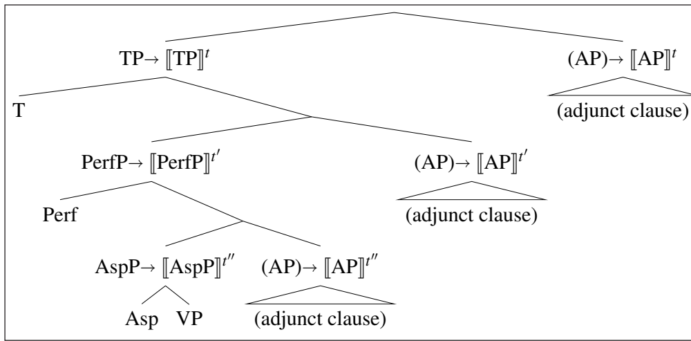
Figure 2 Adjuncts take the evaluation indices of their sisters.
