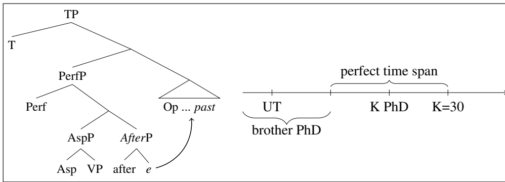
Figure 18 Perfect-level after : adjunct past licensed if the adjunct clause raises to just below T.
