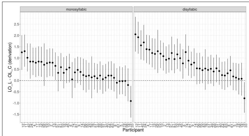
Figure 5: Posterior distribution (mean and 95% CI) of the difference between LO_L and OL_C in derived words (stem level) by participant and stem length (monosyllabic, disyllabic). A positive value means that schwa deletion is more likely in LO_L than in OL_C.
