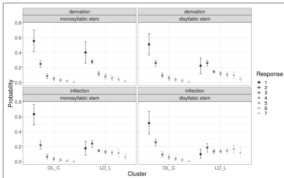
Figure 4: Posterior distribution (mean and 95% CI) of each of the seven response categories as a function of Morphology, Cluster, and Stem Length.
