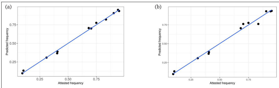
Figure 6: Data vs. predictions for the two grammars. (a) Grammar with *OLC_{der} and *LOL_{der} . (b) Grammar with *CCC_{der} .
