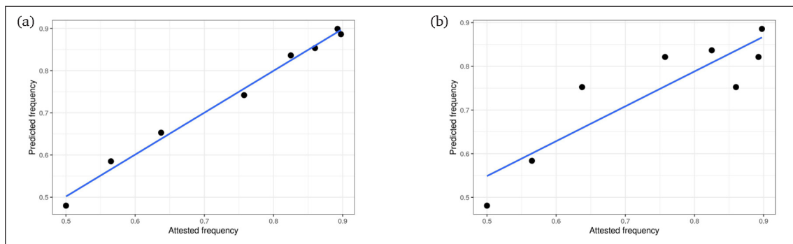
Figure 7: Data vs. predictions for the two grammars. (a) Grammar with *OLC der and *LOL der . (b) Grammar with *CCC der .
